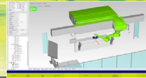
Off-line programming
